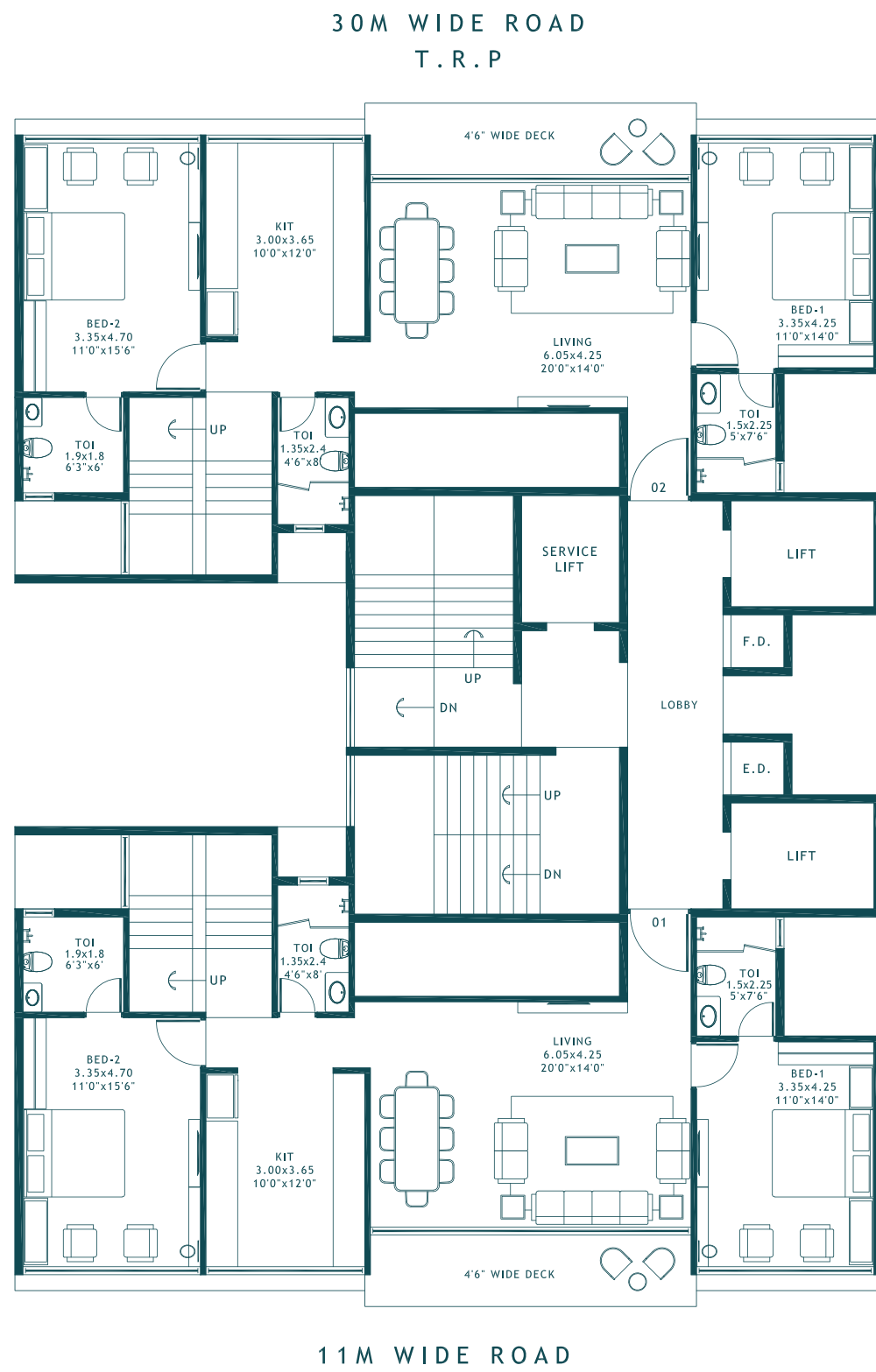
14 th FLOOR PLAN
